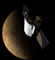
Messenger
