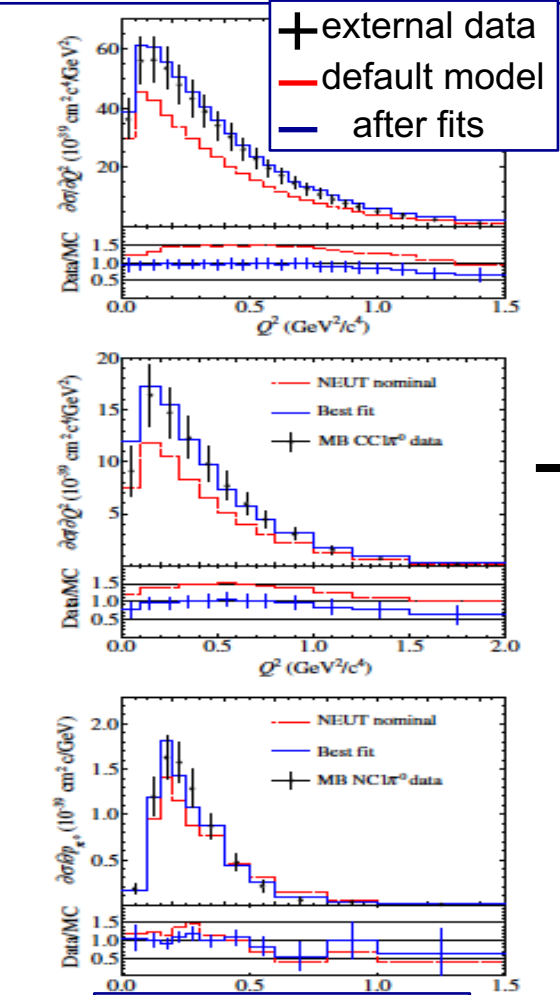
External data fit
