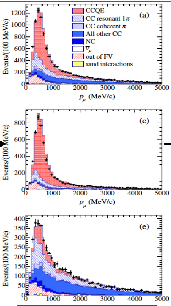
T2K ND280 data fit
