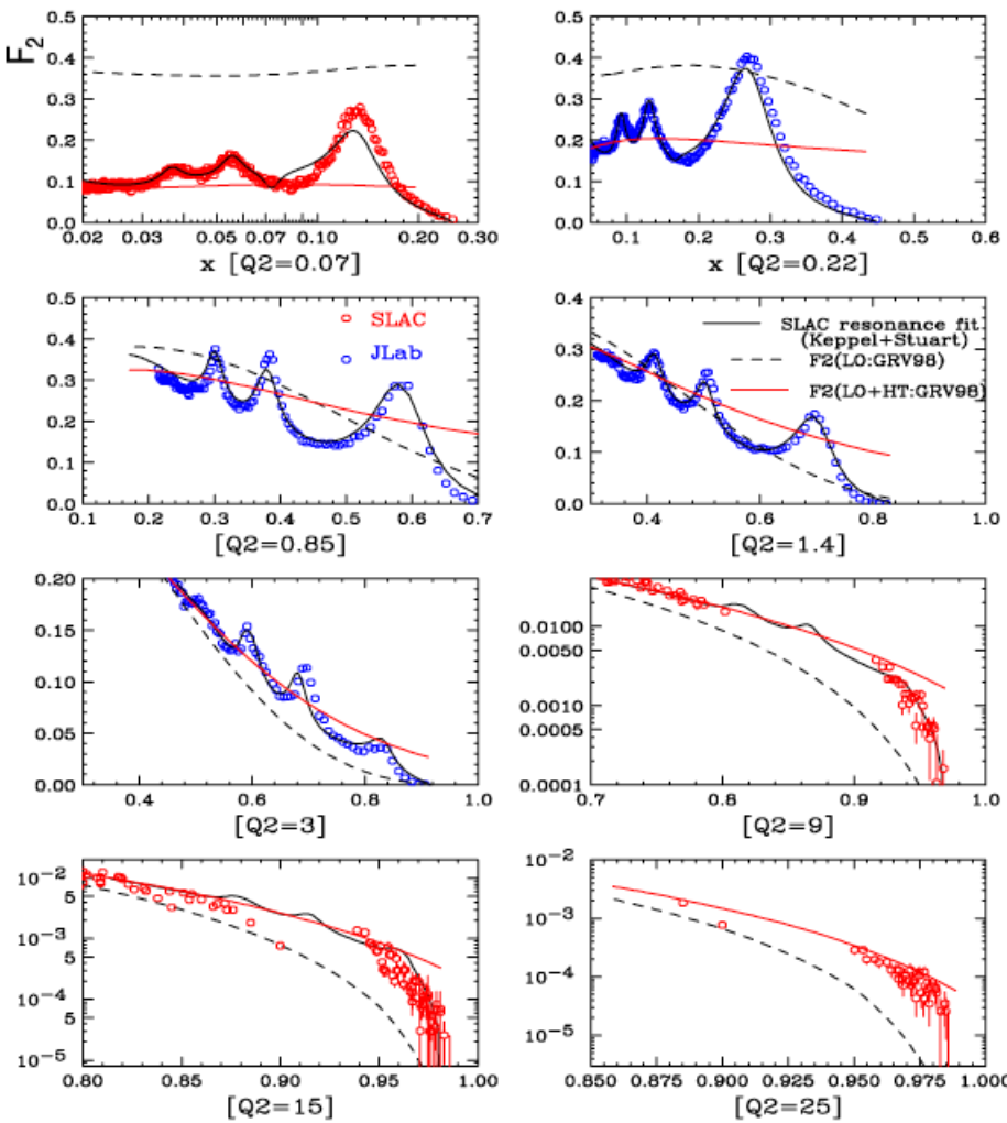
Proton F2 function GRV98-BY correction vs. data
