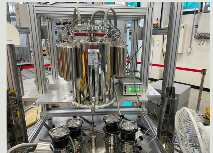
Reliquefier in operation
